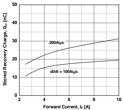
Figure 22. Stored Charge
